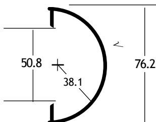
Base: 410540 Endcap: 310206
