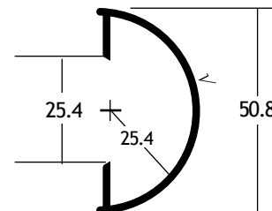
Base: 410443, 410466 Endcap: 310205
