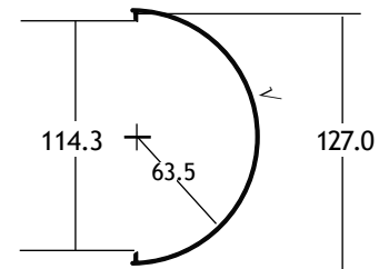
Base: 412002 Endcap: 310208
