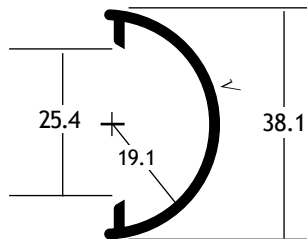
Base: 410443, 410466 Endcap: 310204
